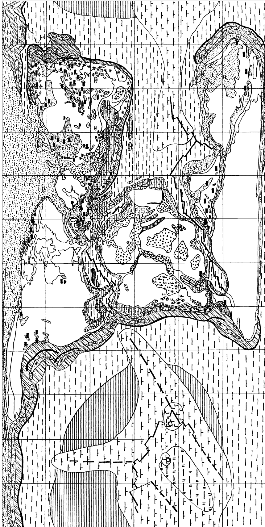
Fig. 3. The lithologic-paleogeographic map for the Hauterivian age of the Cretaceous (symbols as in Fig. 1).
