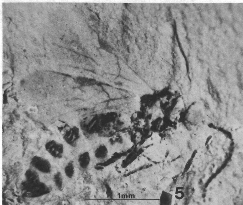
FIG. 5. Eobracon inopinatus Photograph in polarized light.
