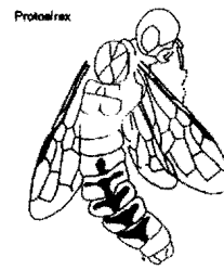
Fig. 8. The primitive hornail Protosirex xyelopterus Rasnitsyn, 1969 (Gigasiricidae) from the Upper Jurassic of South Kazakhstan (after Rasnitsyn, 1969).
