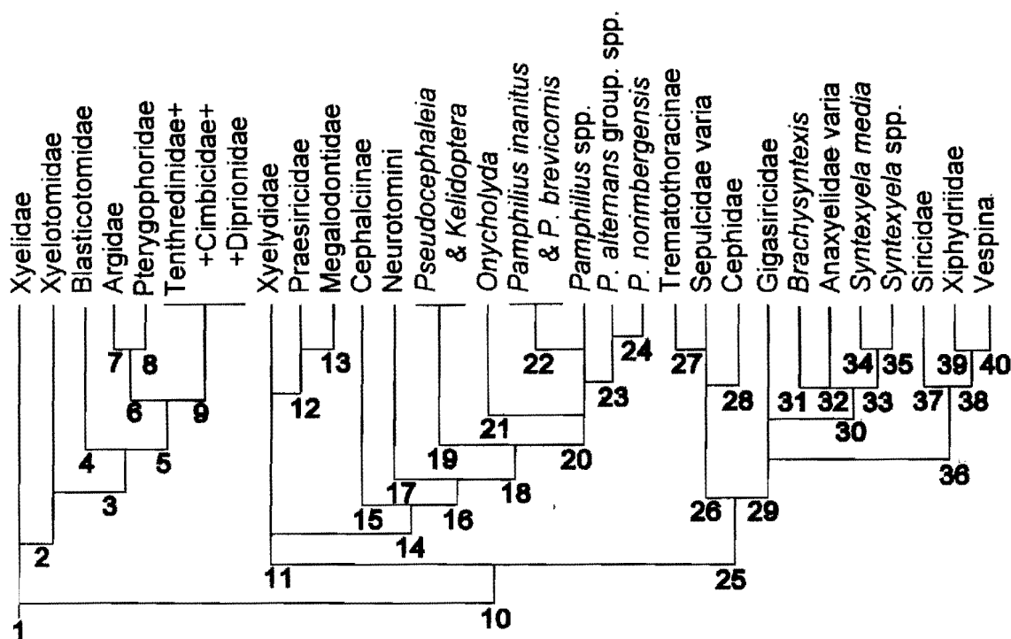
Fig. 12. Cladogram of the lower hymenopterous insects (suborder Siricina) constructed consistent with the hypothesis [(4) in the text] that similarity in the xyeloid antenna is symplesiomorphic, and the alternative similarities are synapomorphic. Otherwise as in Figs. 10–11, with the following synapomorphies inferred:
