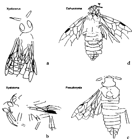
Fig. 5. Representatives of the sawfly family Xyelotomidae: a, Xyelocerus admirandus Rasnitsyn, 1968; b, Xyelotoma nigricornis Rasnitsyn, 1968; c, Pseudoxyela heteroclita Rasnitsyn, 1968 (all from the Upper Jurassic of South Kazakhstan); d, Dahurotoma robusta Rasnitsyn, 1990, Lower Cretaceous of Transbaikalia (a–b after Rasnitsyn, 1969; c, based on Rasnitsyn, 1969, fig. 82, and specimen PIN 2997/650; d, after Rasnitsyn, 1990).
