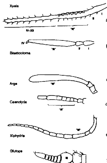
Fig. 3. Antennae of various sawflies, horntails, and flies (unless stated otherwise, of imago): a, Xyela julii Brébisson, 1818 (Xyelidae, pupa); b, Blasticotoma filiceti pacifica Malaise, 1931 (Blasticotomidae); c, Arge ustulata (Linnaeus, 1758) (Argidae); d, Caenolyda reticulata (Linnaeus, 1767) (Pamphiliidae); e, Xiphydria camelus (Linnaeus, 1767) (Xiphydriidae); f, primitive fly Glutops semiformis Nagatomi & Saigusa, 1970 (Rhagionidae) (a–e, after Rasnitsyn, 1968; f, after Nagatomi, 1982). I–XII = segments of antenna, "III" = compound "third" antennal segment.
