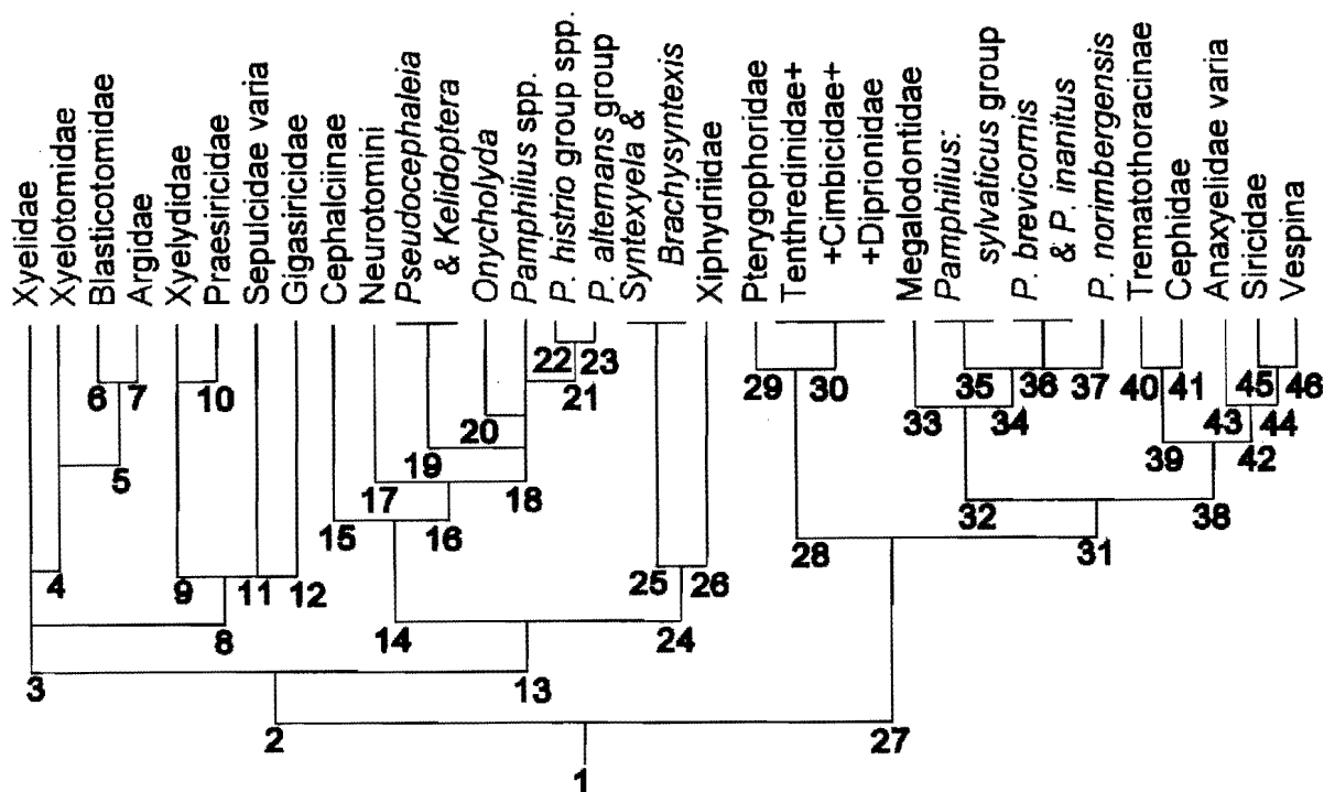
Fig. 10. Cladogram of the lower hymenopterous insects (suborder Siricina) constructed consistent with the hypothesis [(2) in the text] that similarity in the xyeloid antenna is synapomorphic, and the alternative similarities are homoplastic. Figures under the lines of descent refer to the sets of synapomorphies of respective clades (or terminal taxa), as follows (based on Rasnitsyn, 1988a, and, for Pamphiliidae, on Van Achterberg & Van Aartsen, 1986; homoplasies are marked by italics):
