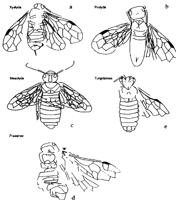
Fig. 6. Representatives of the sawfly families Xyelidae (a–c) and Praesiricidae (d–e): a, Xyelida excellens Rasnitsyn, 1968; b, Prolyda karatavica Rasnitsyn, 1968; c, Mesolyda depressa Rasnitsyn, 1968 (all from the Upper Jurassic of South Kazakhstan); d, Praesirex hirtus Rasnitsyn, 1968; e, Turgidontes magnus Rasnitsyn, 1990 (both from the Lower Cretaceous of Transbaikalia) (a, b, d, after Rasnitsyn, 1983b; c, original, based on holotype; e, after Rasnitsyn, 1990).
