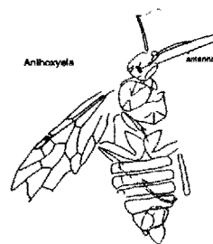
Fig. 2. Anthoxyela turgensis Rasnitsyn, 1990 (Xyelidae); Lower Cretaceous of Transbaikalia (after Rasnitsyn, 1990).
