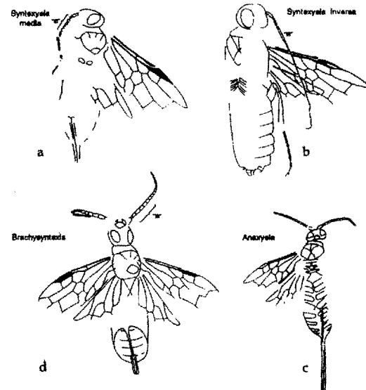
Fig. 9. Representatives of the hornail family Anaxyelidae: a, Syntexyela media (Rasnitsyn, 1963); b, S. inversa Rasnitsyn, 1968; c, Anaxyela gracilis Martynov, 1925; d, Brachysyntexis micrura Rasnitsyn, 1969; all from the Upper Jurassic of South Kazakhstan (a, c, d, after Rasnitsyn, 1969; b, original, based on holotype).
