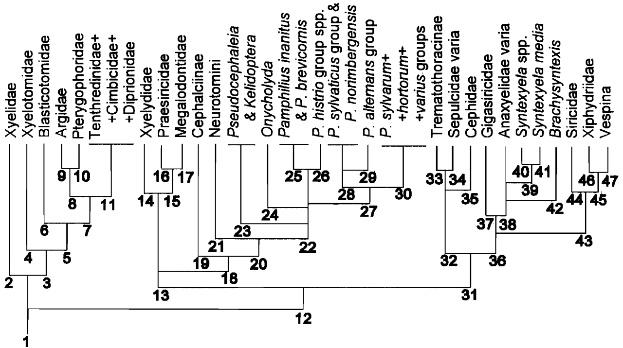
Fig. 11. Cladogram of the lower hymenopterous insects (suborder Siricina) constructed consistent with the hypothesis [(3) in the text] that similarity in the xyeloid antenna is homoplastic, and the alternative similarities are synapomorphic. Otherwise as in Fig. 10, with the following synapomorphies inferred:
