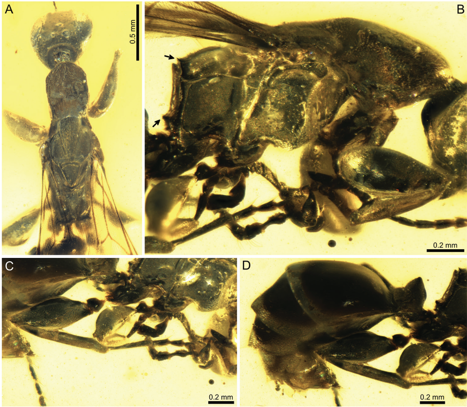
Figure 2. Photographs of Siccibythus robustus sp. nov. (Female holotype; CNU-HYM-MA-2016212) A mesosoma in dorsal view B mesosoma in lateral view, arrowheads indicate metapleural-propodeal boundary, black arrow indicates the carinae C hind leg in lateral view D metasoma in lateral view.
