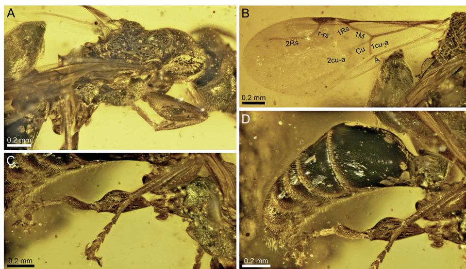
Figure 4. Photographs of Siccibythus robustus sp. nov. (Male paratype; CNU-HYM-MA-2016213) A mesosoma in dorsal view B fore wing venation C hind leg in lateral view D metasoma in lateral view.
