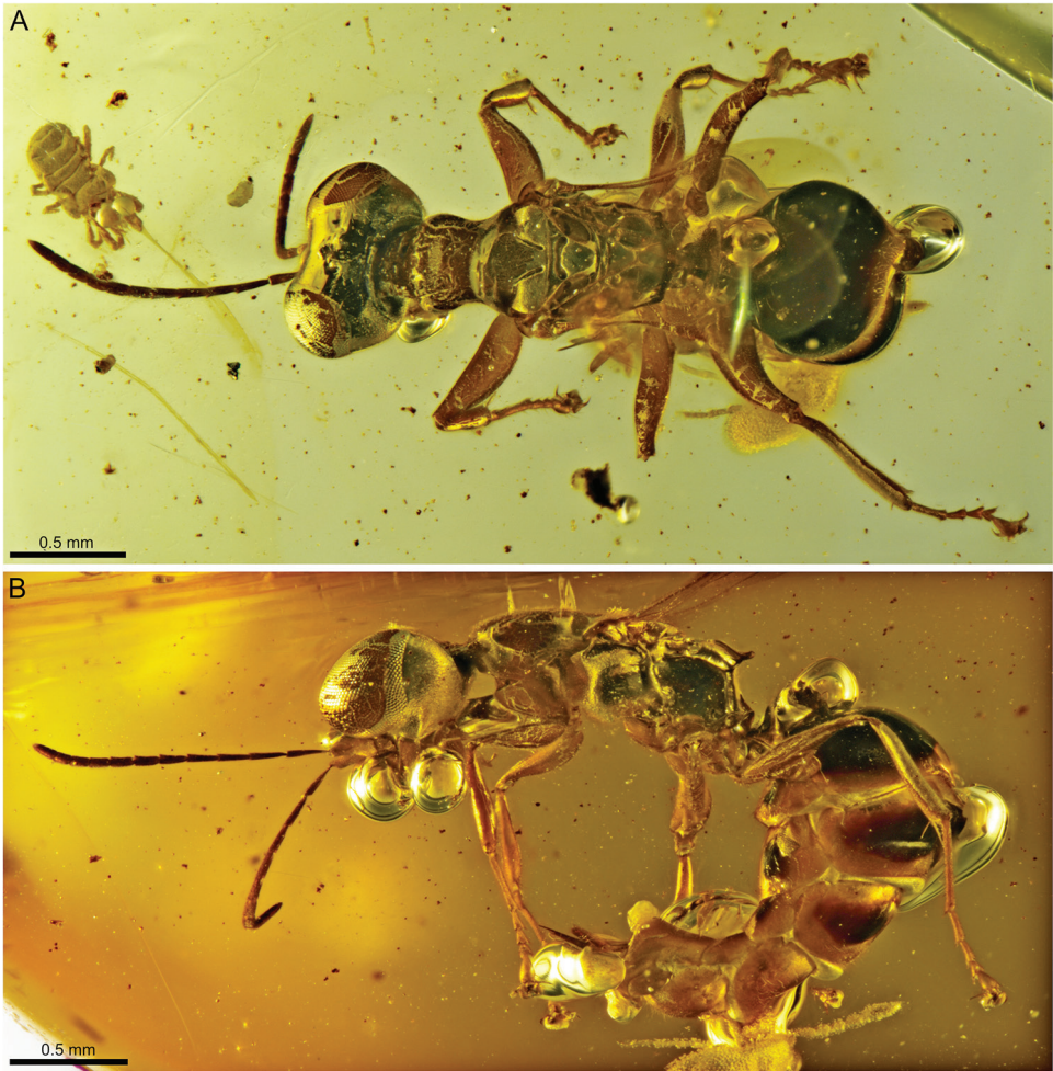
Figure 5. Photographs of Siccibythus aristovi sp. nov. (Female holotype; CNU-HYM-MA-2016214) A habitus in dorsal view B habitus in lateral view.
