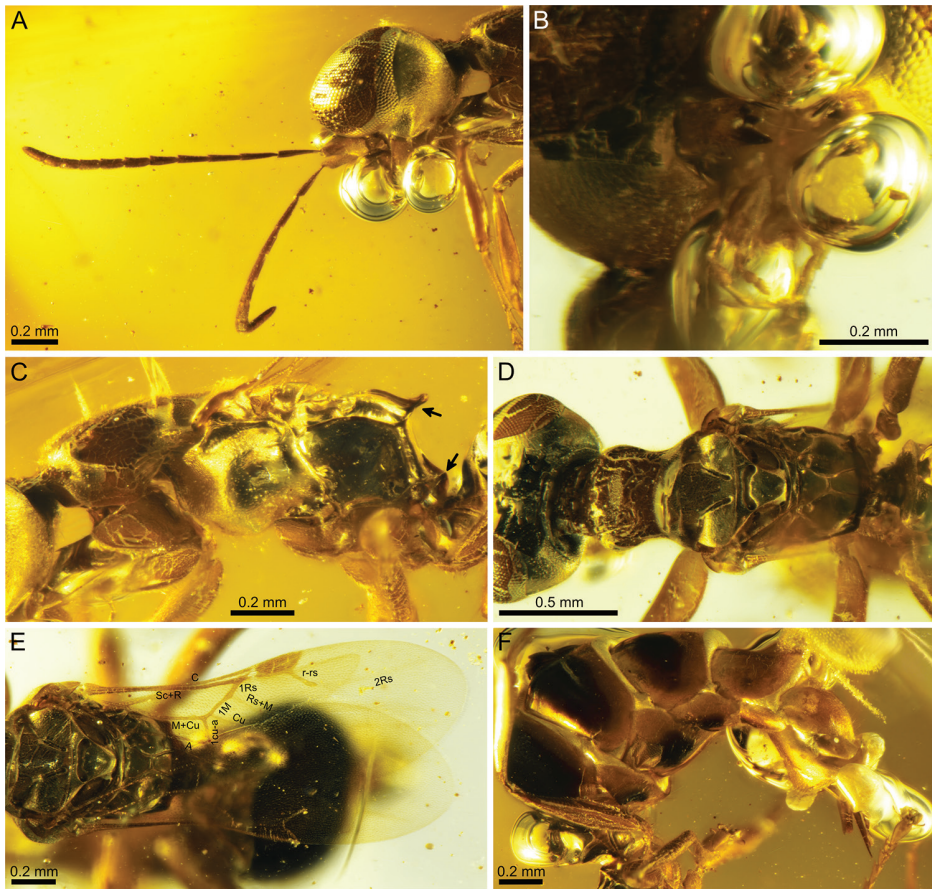
Figure 6. Photographs of Siccibythus aristovi sp. nov. (Female holotype; CNU-HYM-MA-2016214) A head in lateral view B mouthparts C mesosoma in lateral view, black arrow indicates the carinae D mesosoma in dorsal view E fore wing venation F metasoma in lateral view.
